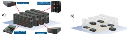
Figure 1: a) Building blocks of modern data center, b) Disaggregated data center architectures
